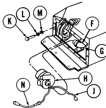
RIGHT CENTRIFUGAL FAN REMOVED FOR CLARITY
